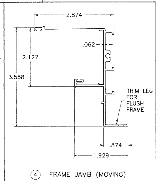
③ FRAME JAMB (MOVING/FIXED)
